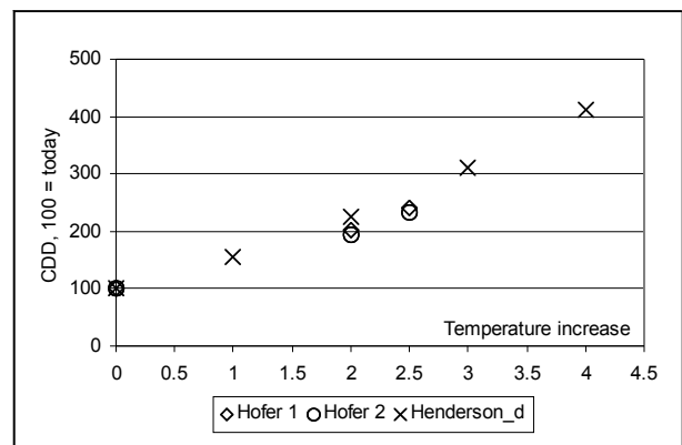
Figure 6. Relative change of Cooling Degree Days (100 = mean temperature today in Switzerland) in the case that temperature increases in summer (June–August) between 1 and 4 °C. (Source: Hofer, Henderson, CEPE)
