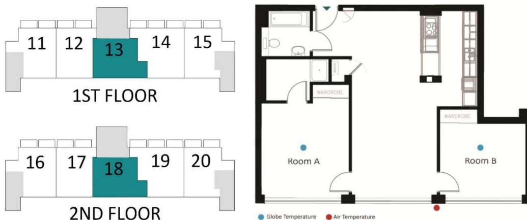
Figure 2. Building floor layout and Unit 13 and 18 layouts with sensor positions.
